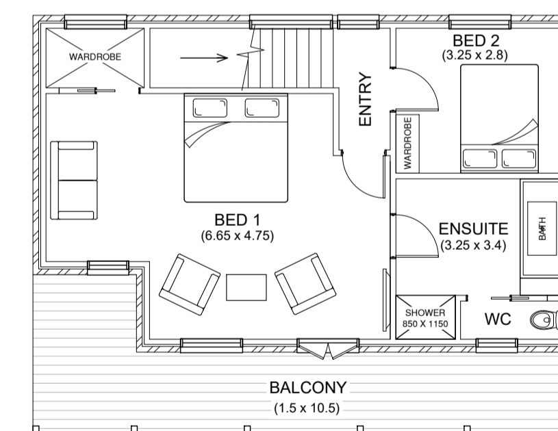
FIRST FLOOR LAYOUT PLAN 1:100
