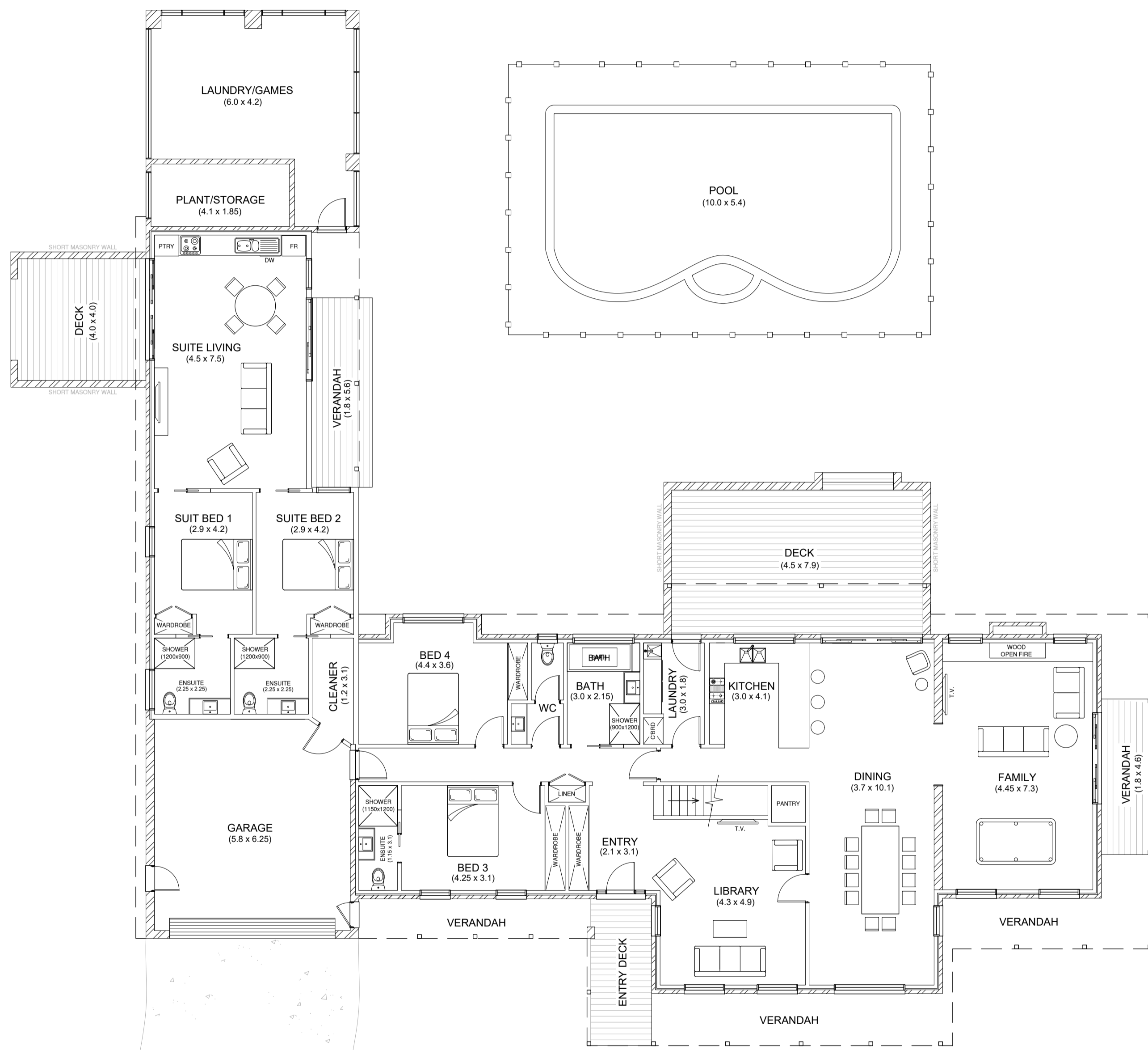
GROUND FLOOR LAYOUT PLAN 1:100
